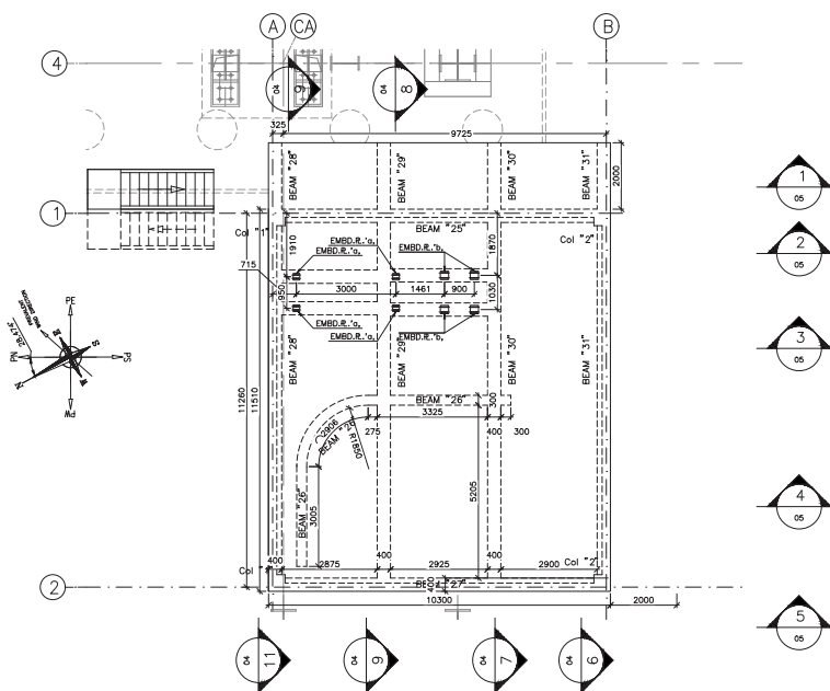
SLAB & WALL FORMWORK PLAN AT ELEV. +16.400
