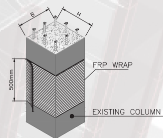
SCHEMATIC VIEW OF RETROFITTED COLUMN
