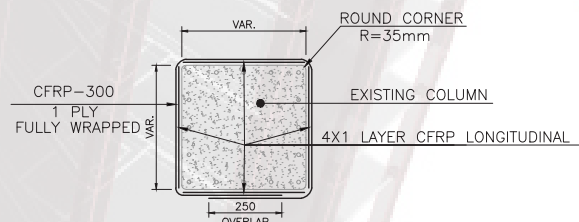
RETROFITTED COLUMN SECTION SEC B
