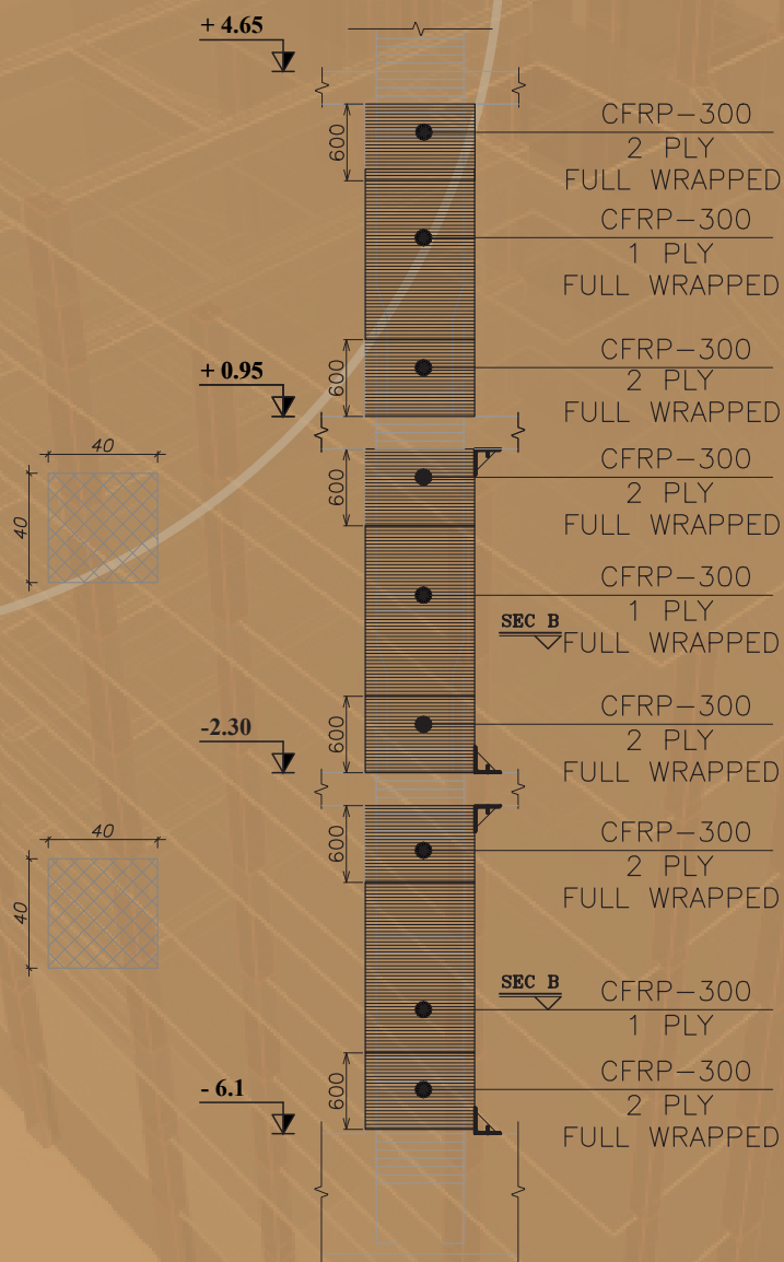
Retrofitted Column F Step2: Transverse Oriented Fibers
