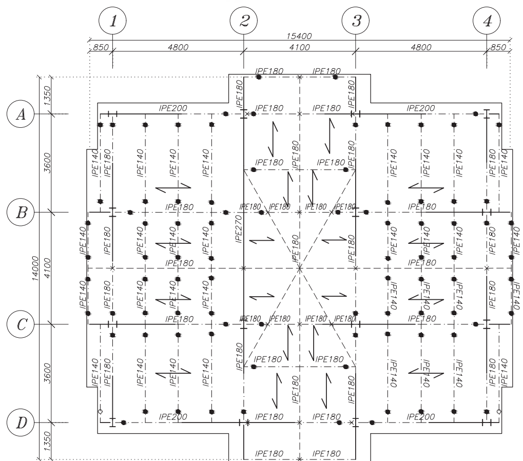
Roof SubStructure Layout
